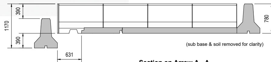
Section on Arrow A - A
